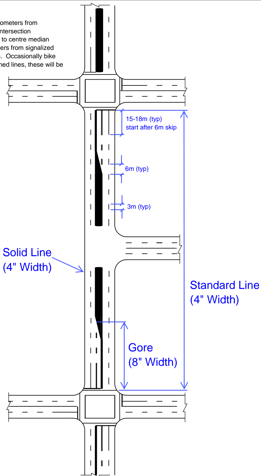
LANE LINES ON TOWAY ROADWAY
